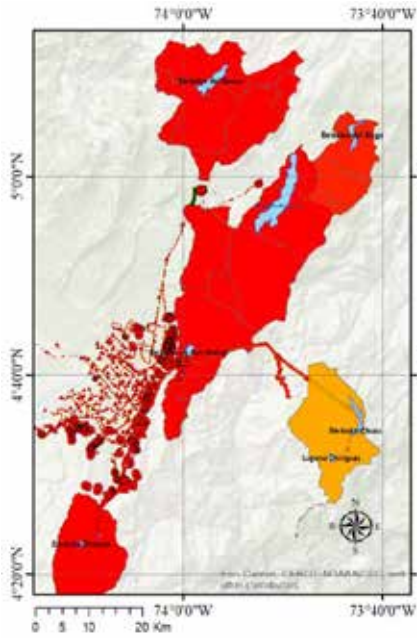
d) Sequía
