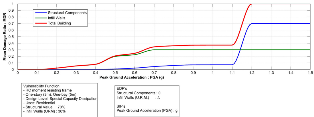
Figure 12. Vulnerability function of the hypothetical building.
